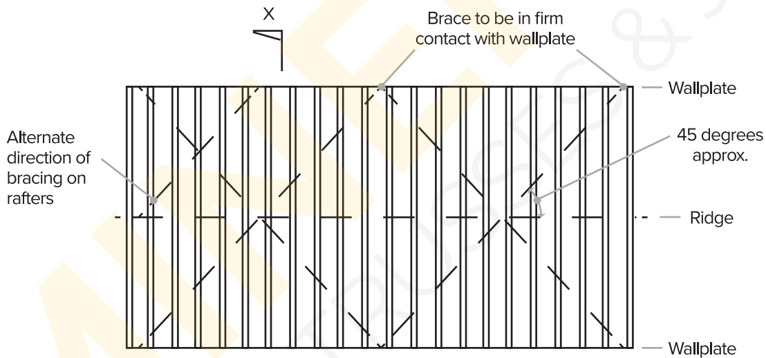
PLAN ON RAFTERS
